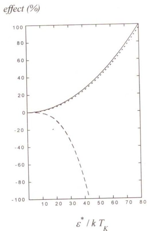
Fig. 1. Predictions of the effect of a temperature gradient on the chemical rate of reaction in dilute gases. The dotted line is the prediction (3.18), which has been calculated in the present paper including all second-order terms and corresponds to the hypothesis that T_K is the measurable temperature. The dashed line corresponds to the calculations in Ref. [5]. The full line includes all second-order terms but corresponds to the assumption that T is the measurable temperature [6] (see Eq. (4.2)), so that in this case the horizontal axis is \varepsilon^*/kT . The reduced temperature gradient is 0.011, corresponding to a temperature gradient of 3.46 \cdot 10^6 K/m (assuming that the temperature is 300 K, n = 2.687 \cdot 10^{25} molecules/m 3 and d = 10^{-10} m).
