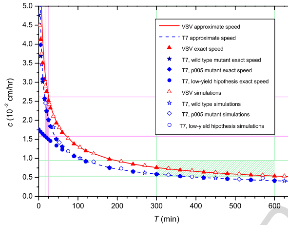
Fig. 1. Focal infections. Front speed versus lag time. The curves stand for the approximate solution c = \sqrt{2D/T} . The solid curve corresponds to VSV ( D = 1.44 \cdot 10^{-4} cm 2 /h) and the dashed curve to the two T7 mutants ( D = 8.55 \cdot 10^{-5} cm 2 /h). The full (empty) symbols correspond to the results of the exact theory (simulations). The triangles represent the results for VSV ( Y = 4983 [11]). The stars stand for the wild T7 strain ( Y = 34.5 [3]), and the rhombus for the p005 T7 mutant ( Y = 63.6 ). The circles represent a hypothetical low-yield case Y = 5 . The hatched (shaded) area corresponds to the observed ranges of T and c for VSV (T7) viruses. Details on the parameter values and the simulations appear in Appendix A.
